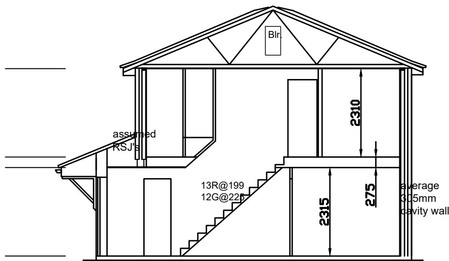
Section X-X
