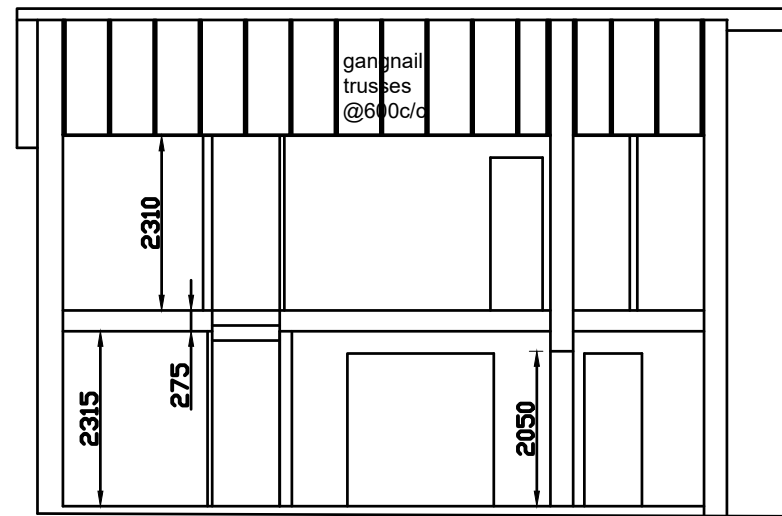
Section Y-Y
