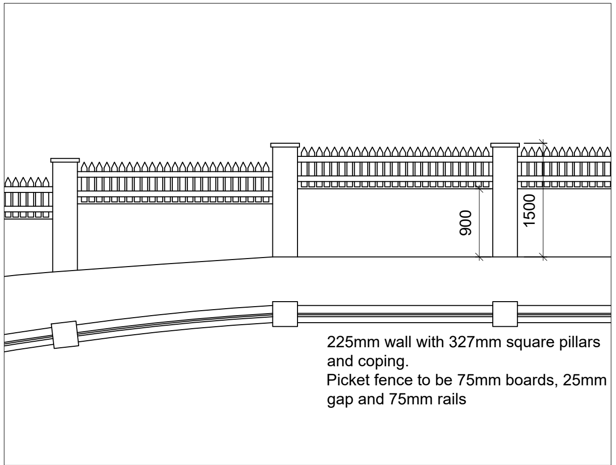
WALL / FENCE DETAIL SCALE - 1:50
