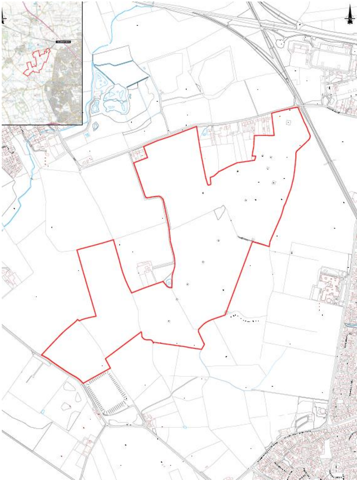
California Farm, Horseclose Lane (Off Letch Lane), Stockton-On-Tees Proposed solar farm (49.9mw) and battery energy storage system (BESS) and associated infrastructure, access and landscaping.
