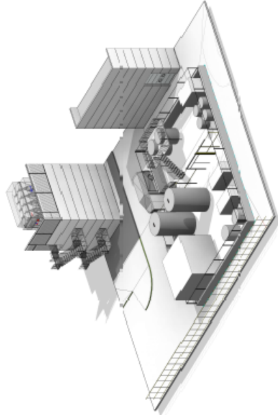
3 3D - LWTP - EXTERNAL VIEW 2
