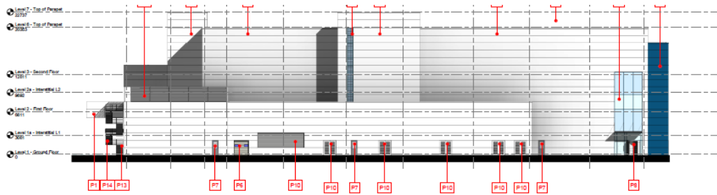
3 North Elevation 1:200
