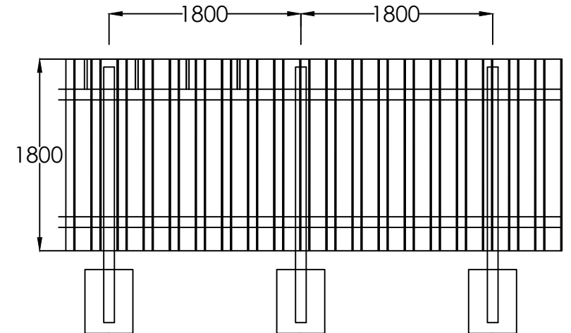
Timber Fence Detail
